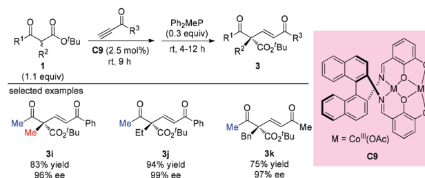
Scheme 13 Asymmetric addition of \beta -ketoesters to alkynes using a Co-Schiff base.
