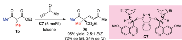
Scheme 11 Asymmetric 1,4-addition of \beta -ketoester to alkyne using catalyst C7 .
