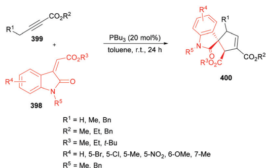
Scheme 101 Regio- and diastereoselective construction of spirocyclopenteneoxindoles through phosphine-catalyzed [3 + 2] annulation of methyleneindolinones with alkyneates.
