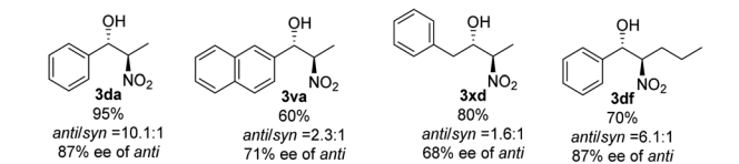
Scheme 36 Cinchona alkaloid catalyst C14 catalyzed Henry reactions.
