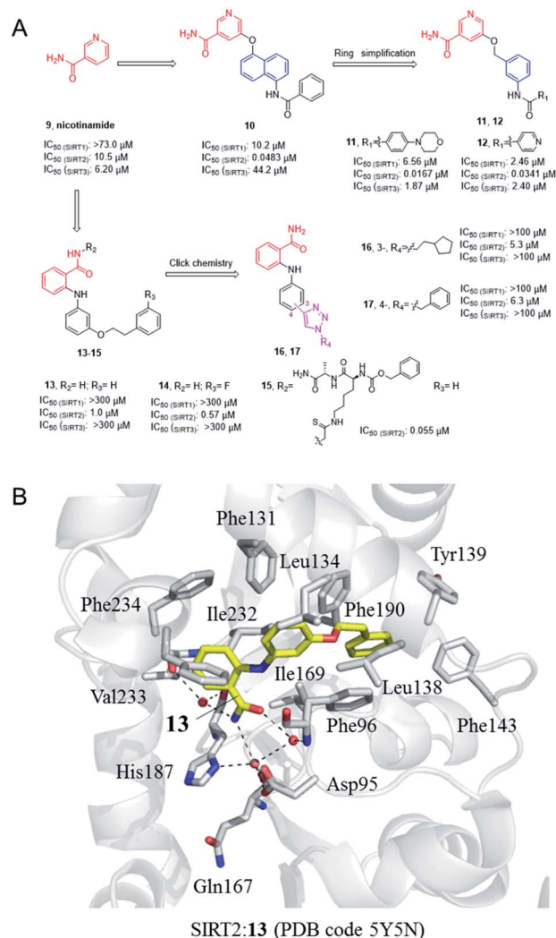
Fig. 3 (A) Chemical structures of nicotinamide-based SIRT2 inhibitors and their inhibitory activity data on SIRT2 determined by Fluor de Lys assays. 34 (B) Crystallographic analyses revealed the binding features of 13 with SIRT2.
