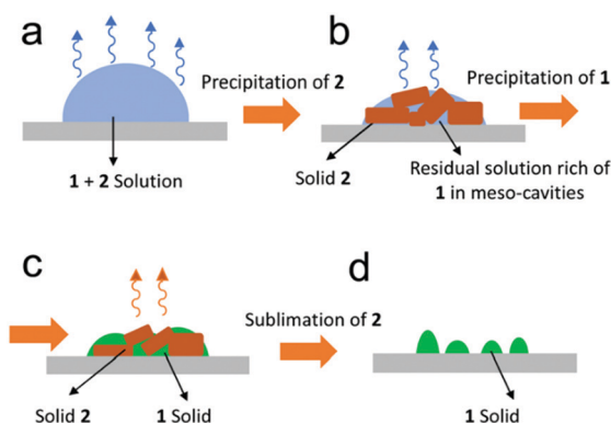
Fig. 15 Scheme of operation of auxiliary solvent based sublimation-aided nanostructuring (ASB-SANS). (a) Drop casting of 1 + 2 solution; (b) precipitation of the overabundant 2; (c) drop precipitation of 1 into the cavities of 2; (d) sublimation of 2. Reproduced from ref. 75 with permission from the Royal Society of Chemistry.
