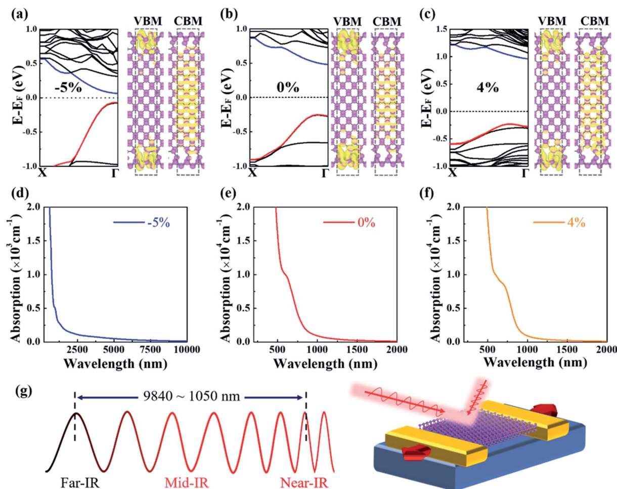
Fig. 5 Electronic band structures of ZZ[Tube] PNRs with a width of 40 Å under strains of -5%, 0% and 4%. The VBM and CBM are highlighted in red and blue, respectively. The isosurface value is 1.2 \times 10^{-4} |e| \text{ bohr}^{-3} (a-c). The VBM and CBM are highlighted in red and blue, respectively. (d)–(f) Optical absorption coefficients of ZZ[Tube] PNRs under strain at -5%, 0% and 4%. (g) A schematic diagram of a possible optoelectronics application of ZZ[Tube] PNRs.
