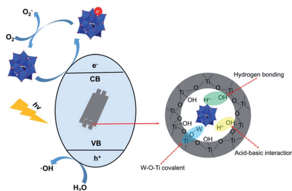
Fig. 4 Structure and photocatalytic mechanism of the \text{H}_3\text{PW}_{12}\text{O}_{40}/\text{TiO}_2 composite material. 74
