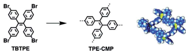
Fig. 13 Synthesis of TPE-CMP with a closed tetragonal skeleton. Reproduced with permission. 141 Copyright 2011, American Chemical Society.
