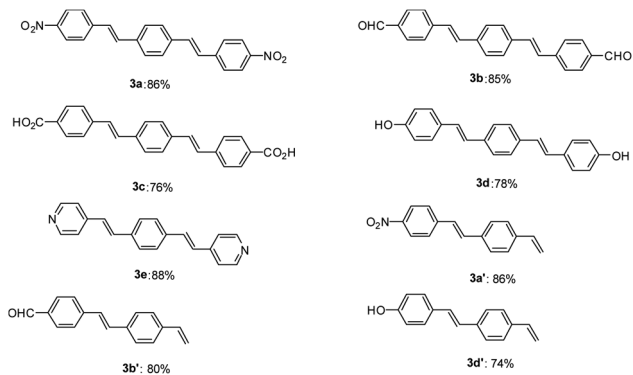
Fig. 1 Synthesis of diverse symmetrical DSBs and vinyl-functionalized stilbenes using Pd–NHC–MIL-101(Cr) catalyst. Reaction conditions for compound (3a–e): 1,4-divinylbenzene (0.55 mmol), aryl halide (1.0 mmol), base (2.0 mmol), amount of catalyst 12.0 mg (1.5 mol%), solvent (5 mL), 12 h at 110 °C. Reaction conditions for compound (3a', 3b' and 3d'): 1,4-divinylbenzene (1.1 mmol), aryl halide (1.0 mmol), base (2.0 mmol), amount of catalyst 12.0 mg (1.5 mol%), solvent (5 mL), 12 h at 110 °C. All yields correspond to the isolated product.
