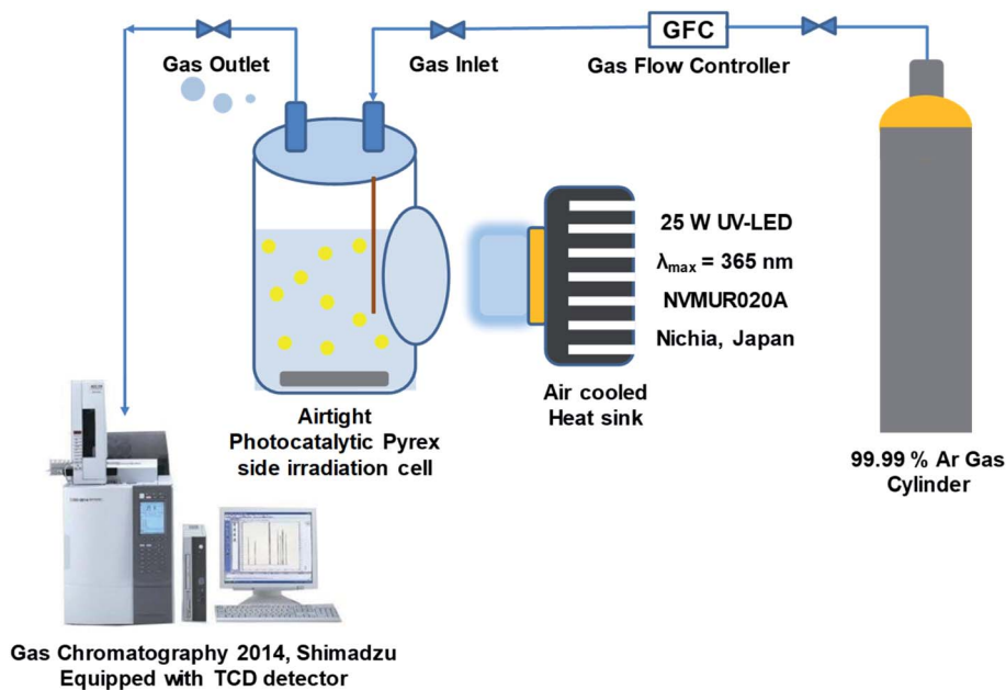
Fig. 2 Photocatalytic hydrogen production flow system.
