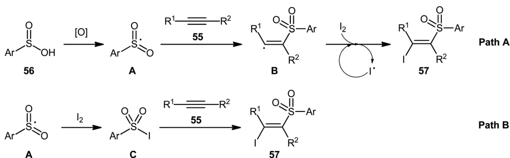
Scheme 25 Possible reaction pathway for the formation ( E )-β-iodovinyl sulfones 57.
