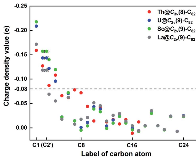
Fig. 12 Charge density values of different carbon atoms in \text{Th}@C_{3v}(8)-C_{82} and M@C_{2v}(9)-C_{82} ( M = \text{U}, \text{Sc}, \text{La} ). Please refer to Fig. 7 for the atom numbering.
