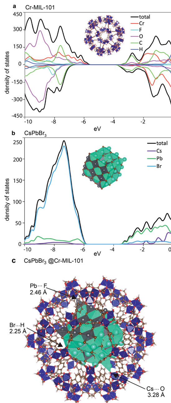
Fig. 6 Electronic density of states calculated for (a) Cr-MIL-101 and (b) nano \text{CsPbBr}_3 . (c) Minimum-energy geometry for \text{CsPbBr}_3 @nano-Cr-MIL-101.
