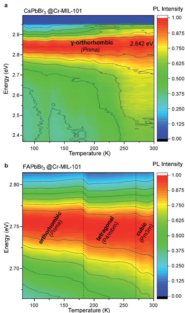
Fig. 5 (a) Photoluminescence evolution over temperature (from 80 to 300 K) for \text{CsPbBr}_3 @nano-Cr-MIL-101. (b) Photoluminescence evolution over temperature (from 80 to 300 K) for \text{FAPbBr}_3 @nano-Cr-MIL-101.
