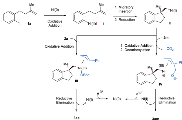
Scheme 4 Proposed mechanism.
