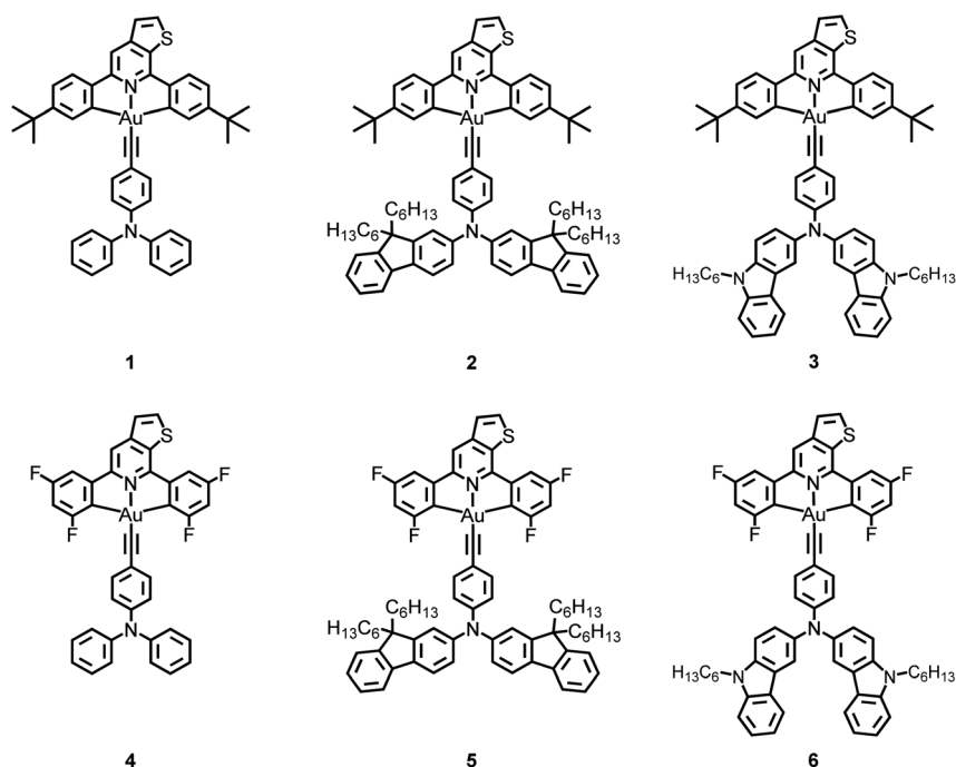
Scheme 1 Molecular structures of the cyclometalated alkyngold(III) complexes 1–6 .
