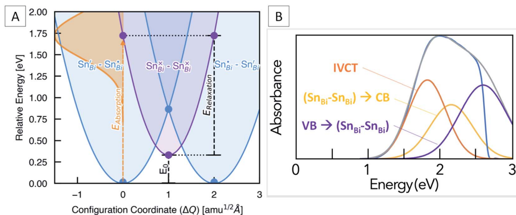
Fig. 5 (A) Configuration coordinate diagram for the (\text{Sn}_{\text{Bi}}^{\cdot}-\text{Sn}_{\text{Bi}}^{\cdot}) to (\text{Sn}_{\text{Bi}}^{\times}-\text{Sn}_{\text{Bi}}^{\times}) IVCT transition, showing the calculated optical excitation ( E_{\text{absorption}} ), vibrational relaxation ( E_{\text{relaxation}} ) and thermodynamic transition ( E_0 ) energies. The solid lines are harmonic fits to the DFT energies, represented by filled circles. X-Axis given in units of mass-weighted displacement. (B) Difference absorption spectrum of Sn doped and undoped \text{Cs}_3\text{Bi}_2\text{Br}_9 , fitted with three components corresponding to the IVCT absorption and two 'band to band gap state' transitions at energies calculated from DFT.
