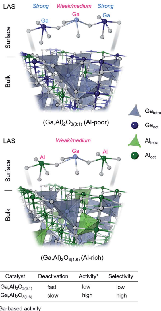
Fig. 5 Schematic representation of the distribution of bulk metal sites ( M_{IV} and M_{VI} , M = \text{Ga, Al} ) in (\text{Ga, Al})_2\text{O}_{3(3:1)} and (\text{Ga, Al})_2\text{O}_{3(1:6)} catalysts as well as the representative surface sites in these materials. The nature of surface metal sites and their Lewis acidity is linked to their performances in PDH.
