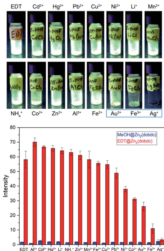
Fig. 5 (a) Dry samples of EDT loaded \text{Zn}_2(\text{dobdc}) after 24 h soaking in solution of metal cations. (b) Graph of the fluorescence intensity of the samples (red bars). The corresponding results of a control experiment with methanol solvated \text{Zn}_2(\text{dobdc}) are presented as blue bars.
