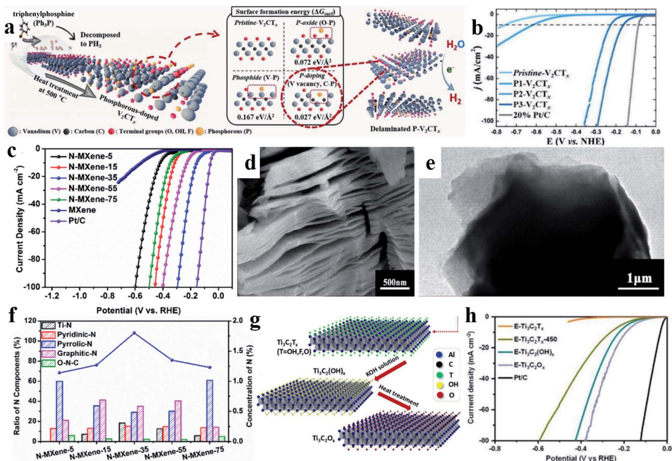
Fig. 11 (a) Synthesis of P- V_2CT_x , reprinted with permission from ref. 128 , Copyright (2019) Wiley-VCH Verlag GmbH & Co. KGaA, Weinheim for (a) and (b); (b) linear sweep voltammetry without iR correction of the sample electrocatalysts with a scan rate of 10 mV s^{-1} ; (c) LSV curves of N- Ti_3C_2T_x at different temperatures and Pt/C at a speed rate of 5 mV s^{-1} ; SEM (d) and TEM (e) images of N- Ti_3C_2T_x -35; (f) comparison of the N content of different N species in N- Ti_3C_2T_x at different temperatures, reprinted with permission from ref. 66 , Copyright (2020) Elsevier B.V. for (c)–(f); (g) schematic illustration of the further process of Ti_3C_2T_x MXene to prepare E- Ti_3C_2O_x ; (h) polarization curves of samples on the GC electrode at 5 mV s^{-1} in 0.5 M H_2SO_4 , reprinted with permission from ref. 130 , Copyright (2018) John Wiley & Sons, Inc. for (g) and (h).
