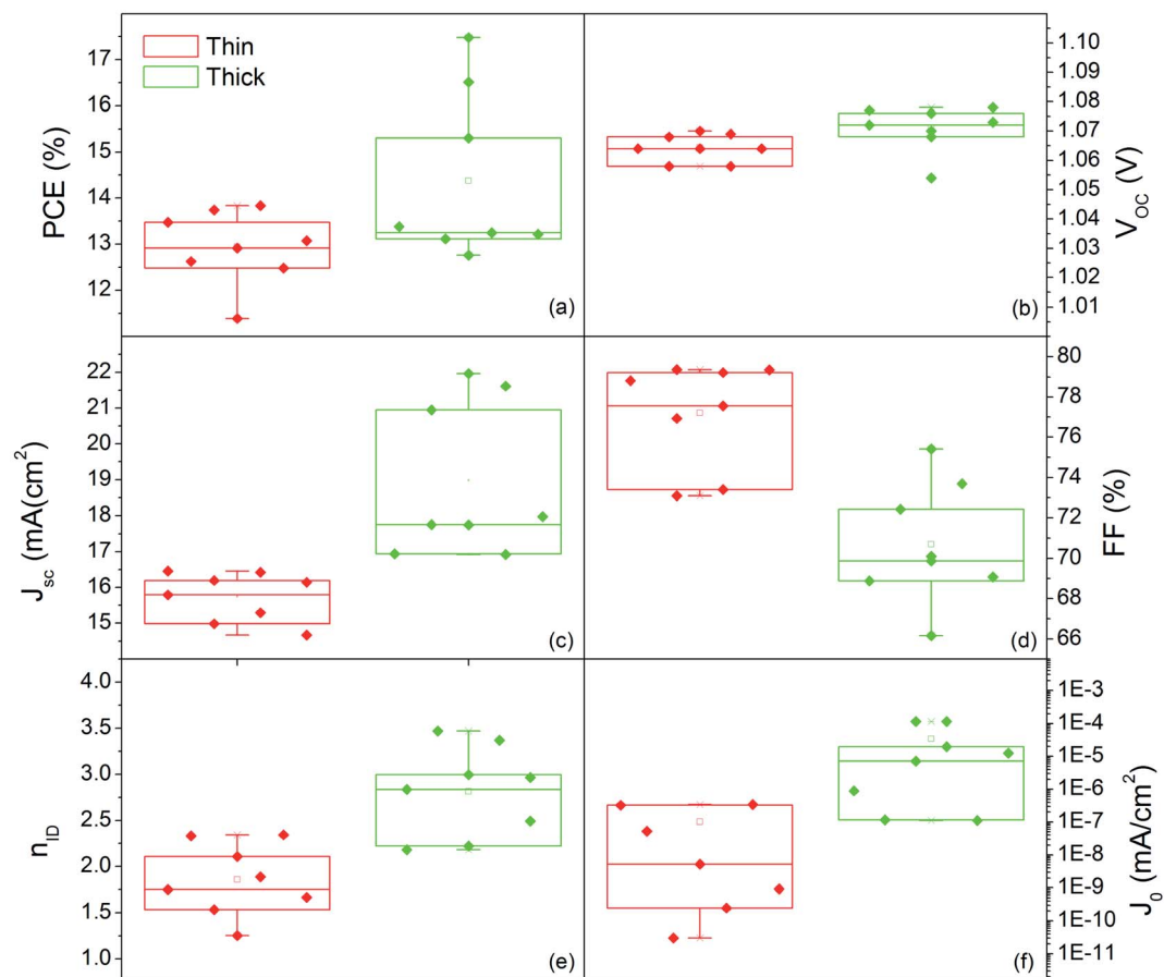
Fig. 10 Box plot of (a) efficiency (PCE), (b) open circuit voltage ( V_{oc} ), (c) short circuit current ( J_{sc} ), (d) fill factor (FF), (e) ideality factor ( n_{ID} ) and (f) reverse saturation current ( J_0 ) from the electrical characterization of all the prepared devices with 80 nm thick and 150 nm thick MAPbI 3 active layers.
