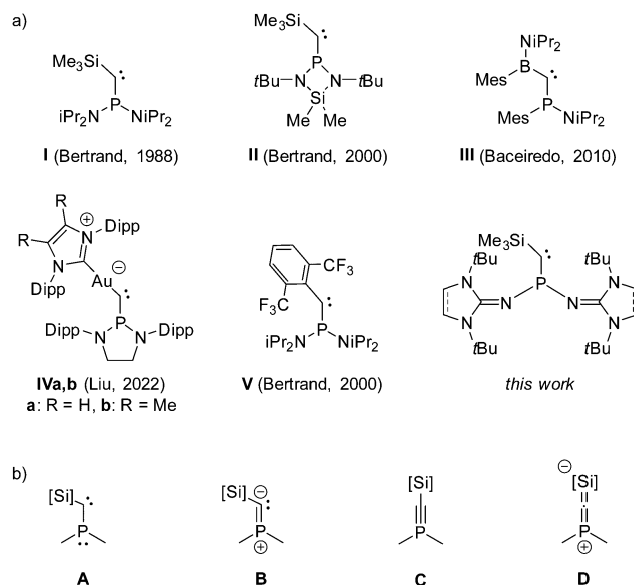
Fig. 1 (a) Selected examples of phosphino(silyl)carbenes and the phosphino(silyl)carbene presented in this work. Dipp = 2,6-diisopropylphenyl. (b) Possible electronic structures of phosphino(silyl)carbenes ([Si] = silyl group).
