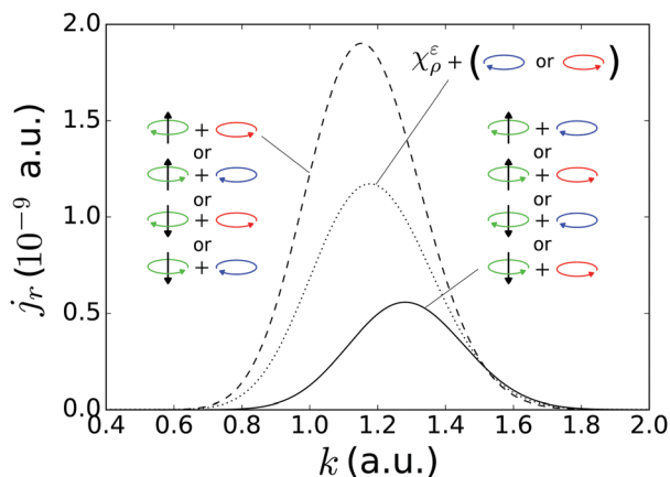
Fig. 3 Radial component of the photoelectron current density (ionization rate) as a function of photoelectron momentum, resulting from strong field ionization of the initial states \chi_c^\epsilon and \chi_c^{\epsilon*} [see eqn (2)–(4) and Fig. 2(a)], via intense light circularly polarized in the xy plane. Up to k \approx 1.5 a.u. all the counter-rotating setups, where the azimuthal part of the bound probability current and the light rotate in opposite directions, yield a higher j_r . Beyond k \approx 1.5 a.u. the co-rotating setups yield a higher j_r . The corresponding curve for the states \chi_\rho^\epsilon is simply the average between the two curves shown and is independent of enantiomer and light polarization. The parameters, \epsilon , \omega , and I_p are the same as in Fig. 2.
