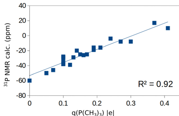
Fig. 4 Plot of computed ^{31}\text{P} chemical shift versus the Bader charge on \text{P}(\text{CH}_3)_3 adsorbed on various \text{M}^{4+} sites of \text{a-TiO}_2 , \text{r-TiO}_2 , \text{ZrO}_2 , \text{SnO}_2 , and \text{CeO}_2 . We also include in the plot the free \text{P}(\text{CH}_3)_3 molecule, with chemical shift -60 ppm and q(\text{P}(\text{CH}_3)_3) = 0 .
