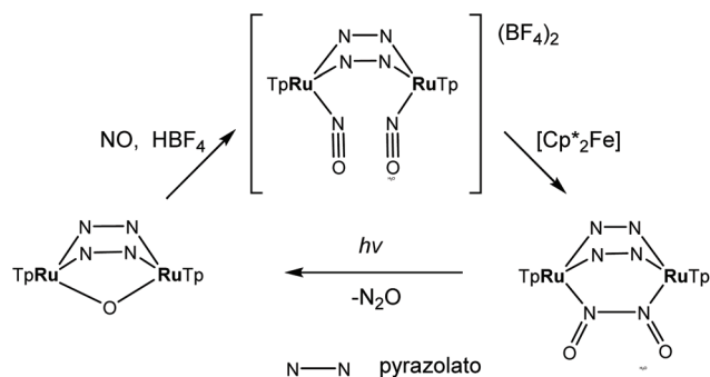
Scheme 4 Synthesis of [\{\text{TpRu}(\text{NO})\}_2(\mu\text{-p-z})_2](\text{BF}_4)_2 and photo-induced conversion of the N–N coupled complex into oxido-bridged starting complex [\{\text{TpRu}(\mu\text{-O})(\mu\text{-p-z})_2\}] .
