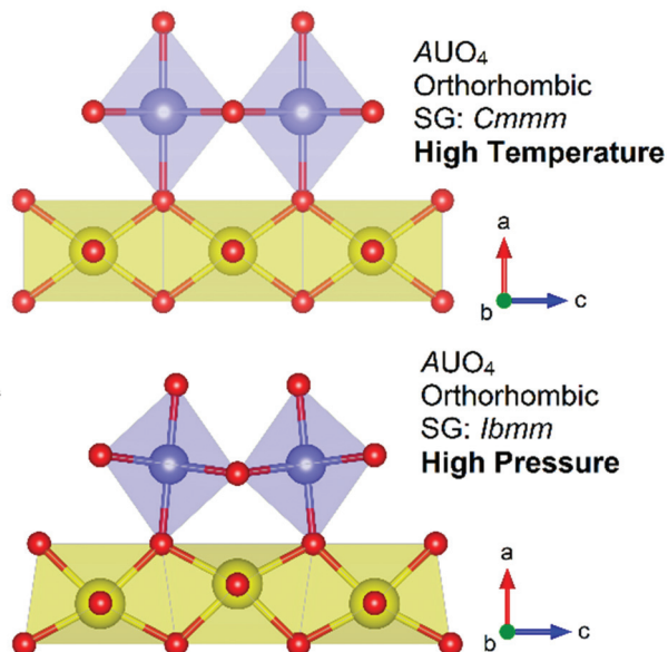
Fig. 9 Structural representations of the AUO_4 orthorhombic structures in space groups Cmmm and Ibmm where it has been shown 3 high temperatures favour the Cmmm structure non-distorted structure and high pressures favour the distorted Ibmm structure. Note the tilt in the AO_6 polyhedra (purple) and distortion of UO_6 polyhedra (yellow) w.r.t. oxygen atoms (red spheres).
