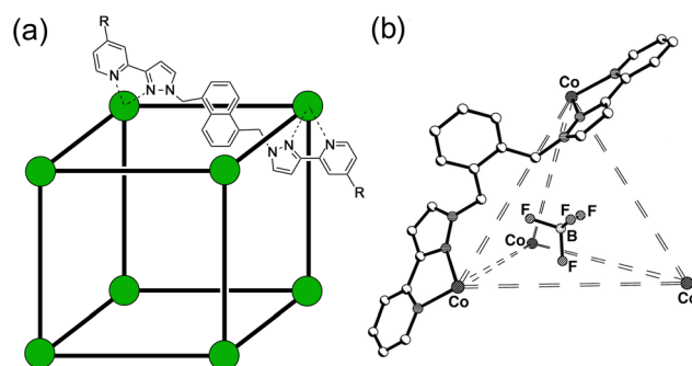
Fig. 1 (a) The cages \text{H}^{\text{W}} [R = CH 2 OH, Co(II) vertices] used for solution studies, and \text{H}^{\text{Ni}} [R = H, Ni(II) vertices] used for the crystallography; and (b) T (used for control experiments).
