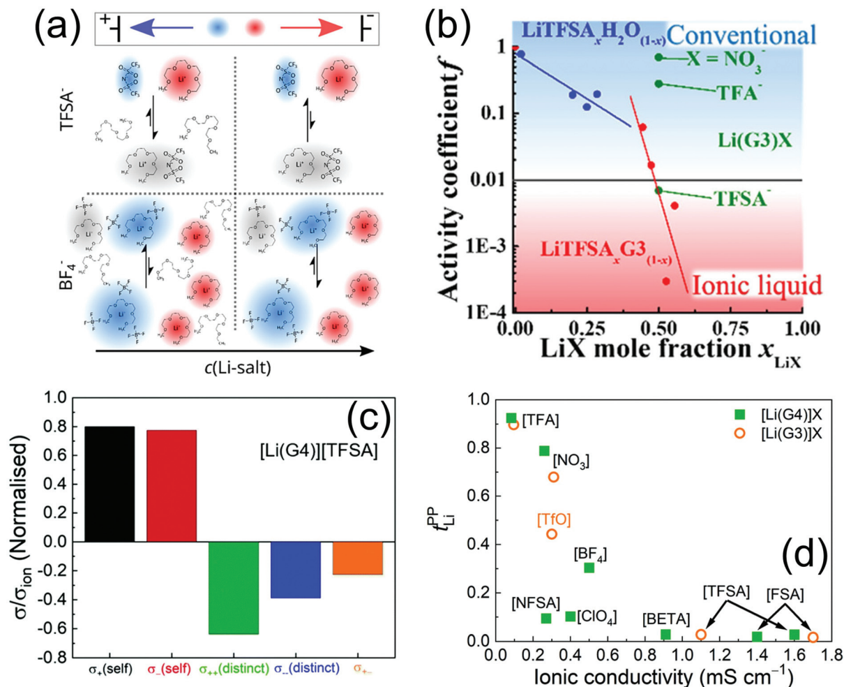
Fig. 6 (a) Schematic representation of speciation: suggested dominant ion clusters in the low and high salt concentration regimes for [\text{Li(G}_4\text{)}]\text{X} (top) and [\text{Li(G}_4\text{)}][\text{BF}_4] (bottom). Anionic species are depicted in blue, cationic species in red, and neutral species in gray. Reproduced with permission. 79 Copyright © 2020 American Chemical Society. (b) Plots of activity coefficients vs. Li salt mole fraction. Blue and red denote [\text{LiTFSI}]_x(\text{H}_2\text{O})_{1-x} and [\text{LiTFSI}]_x(\text{G}_3)_{1-x} , respectively, and green denotes [\text{LiX}][\text{G}_3] ( X = \text{NO}_3^- , \text{TFA}^- , or \text{TFSI}^- ); f < 0.01 is herein used as a thermodynamic criterion for categorizing the mixture as an SIL instead of a concentrated electrolyte solution. Reproduced with permission. 80 © 2020 American Chemical Society. (c) Five transport coefficients according to the Onsager formalism [ \sigma_+(\text{self}) , \sigma_-(\text{self}) , \sigma_{++}(\text{distinct}) , \sigma_{--}(\text{distinct}) , and \sigma_{+-} : left to right] normalized by the ionic conductivity ( \sigma_{\text{ion}} ) of the molten Li salt solvates for the [\text{Li(G}_4\text{)}][\text{TFSI}] complex. Adapted with permission. 81 This journal is © the Owner Societies 2020. (d) Plots of the \text{Li}^+ transference number based on potentiostatic polarization measurements ( t_{\text{Li}}^{\text{PP}} ) vs. ionic conductivity for [\text{Li(G}_n\text{)}]\text{X} complexes ( n = 3 and 4 ; X = \text{TFA} , \text{NO}_3 , \text{Tf} , \text{BF}_4 , \text{NFSI} , \text{ClO}_4 , \text{BETA} , \text{TFSI} , and \text{FSI} ). Reproduced with permission. 82 This journal is © the Owner Societies 2021.
