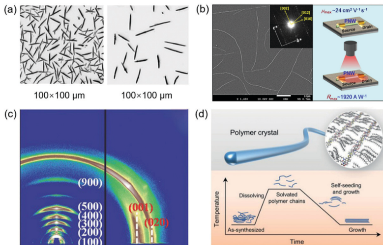
Fig. 13 Conjugated polymer crystals. (a) Optical micrographs of the single crystals of P3HT-26. Reproduced with permission. 176 Copyright 2012, Wiley-VCH. (b) Polymer nanowires of DPPBT SPE and its applications in electronic devices. Reproduced with permission. 65 Copyright 2015, American Chemical Society. (c) GIXRD patterns of poly-PCDA crystals. Reproduced with permission. 178 Copyright 2017, Wiley-VCH. (d) 3D schematic of the polymer crystals by a self-seeding approach. Reproduced with permission. 66 Copyright 2021, Wiley-VCH.
