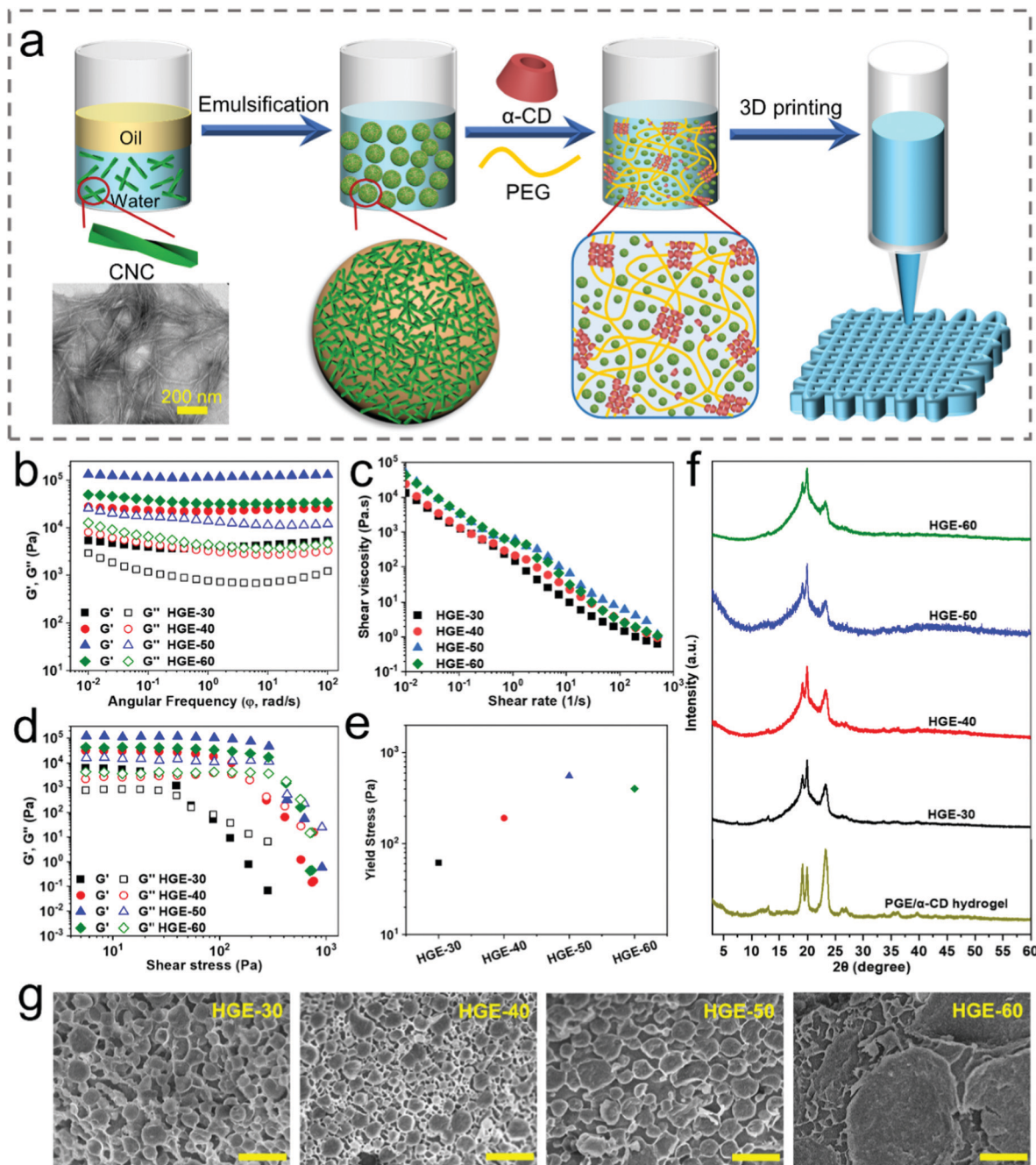
Fig. 1 (a) Schematic illustration of the fabrication of the emulgels using sunflower oil as the dispersed phase for DIW, including the precursor emulgels (emulgels-X) and the host-guest emulgels (HGE-Y), where X and Y refer to the oil fraction. (b) Frequency sweep of the HGEs with different oil phase fractions. (c) Steady state flow curves and (d) stress sweep profiles for the HGEs with different oil phase fractions, as noted. (e) Shear yield stress of the HGE inks. (f) X-Ray diffraction patterns of the HGEs with different oil phase fractions and that of the \alpha -CD/PEG hydrogel synthesized with a molar ratio of the PEG repeat unit to \alpha -CD of 30/1. (g) Cryo-scanning electron microscopy (Cryo-SEM) images of the HGEs with different oil phase fractions. Scale bar: 5 \mu m.
