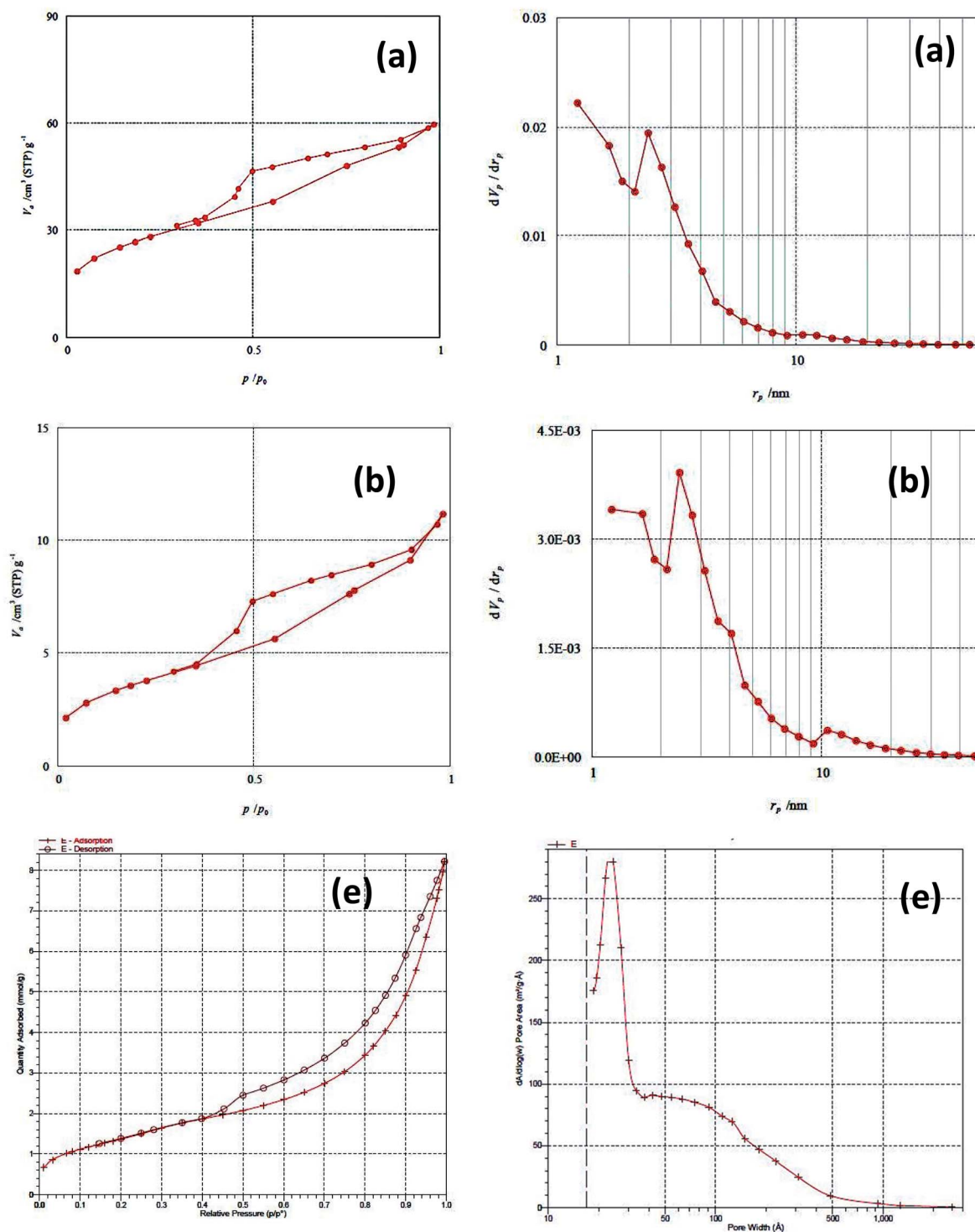
Fig. 4 \text{N}_2 adsorption-desorption isotherms of PMAMOSa,b,e (I) obtained using the PMDADA precursor I prepared in THF (a) or DMF solvent (b) with the simultaneous addition of precursor I and TEOS to the mixture of HCl and Pluronic P123. CTAB was dissolved in ammonia solution and used as the template (e).
