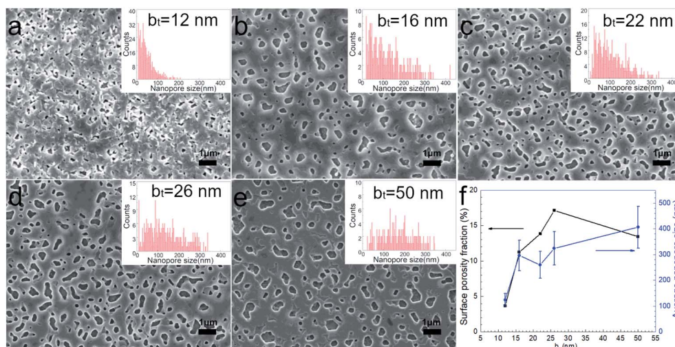
Fig. 5 (a–e) SEM images from annealed \text{Ca(OH)}_2/\text{Co}_3\text{O}_4 multilayers with 12 \leq b_l \leq 50 nm grown on mica (001) substrates. (f) Surface porosity fraction determined from SEM image analyses.
