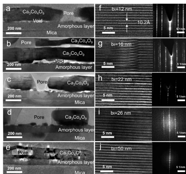
Fig. 6 (a–e) Cross-sectional bright-field TEM images from \text{Ca}_3\text{Co}_4\text{O}_9 films obtained by annealing \text{Ca(OH)}_2/\text{Co}_3\text{O}_4 multilayers with 12 \leq b_l \leq 50 nm created from \text{CaO}/\text{Co}_3\text{O}_4 multilayers. (f–j) The corresponding high-resolution TEM images and SAED patterns capturing the layered atomic structure of \text{Ca}_3\text{Co}_4\text{O}_9 .
