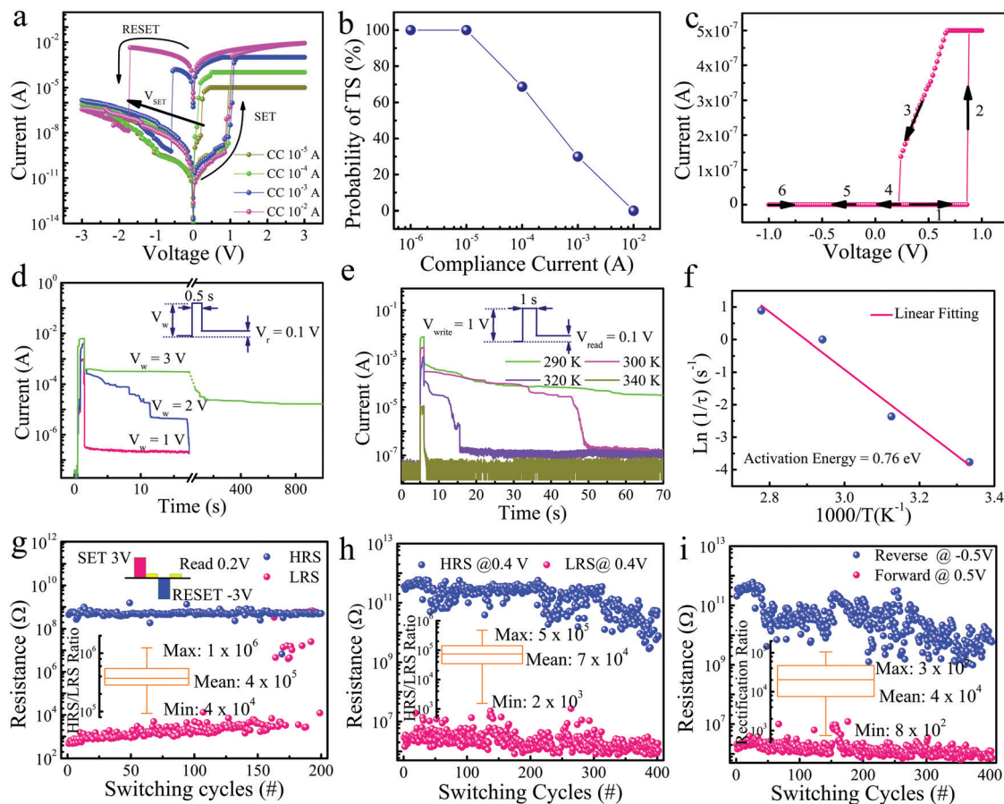
Fig. 2 Systematic analysis on resistive switching. (a) Typical I-V curve of the device under different compliance currents (CCs). (b) Probability for volatile TS as a function of CC, demonstrating the transition from volatile TS to non-volatile MS as increasing the CC. (c) Typical I-V curve of the device under a linear scale over the sweep voltage of -1 V to 1 V. (d) Retention time under different voltage amplitudes. (e) Retention time under different temperatures. (f) The Arrhenius plot of the retention time depending on the temperature. (g) Non-volatile switching under a pulsed-voltage operation. The operation voltage pulse was \pm 3 V with a duration of 1 s. The read voltage was 0.2 V. The duty cycle of the pulse was 50\% . The box plot was based on the first 165 cycles. (h) The HRS/LRS resistance distribution over 400 switching cycles. The data was extracted from the result of the DC switching cycle test. The sweep voltage was -1 V to 1 V, the read voltage was 0.4 V. (i) The distribution of the device resistance under forward and reverse biasing over 400 switching cycles. The data was extracted from the result of the DC switching cycle test. After the device is SET to LRS, read the current at 0.5 V to get the forward resistance. After the device is RESET to HRS, read the current at -0.5 V to get the reverse resistance. The rectification ratio is (reverse resistance)/(forward resistance).
