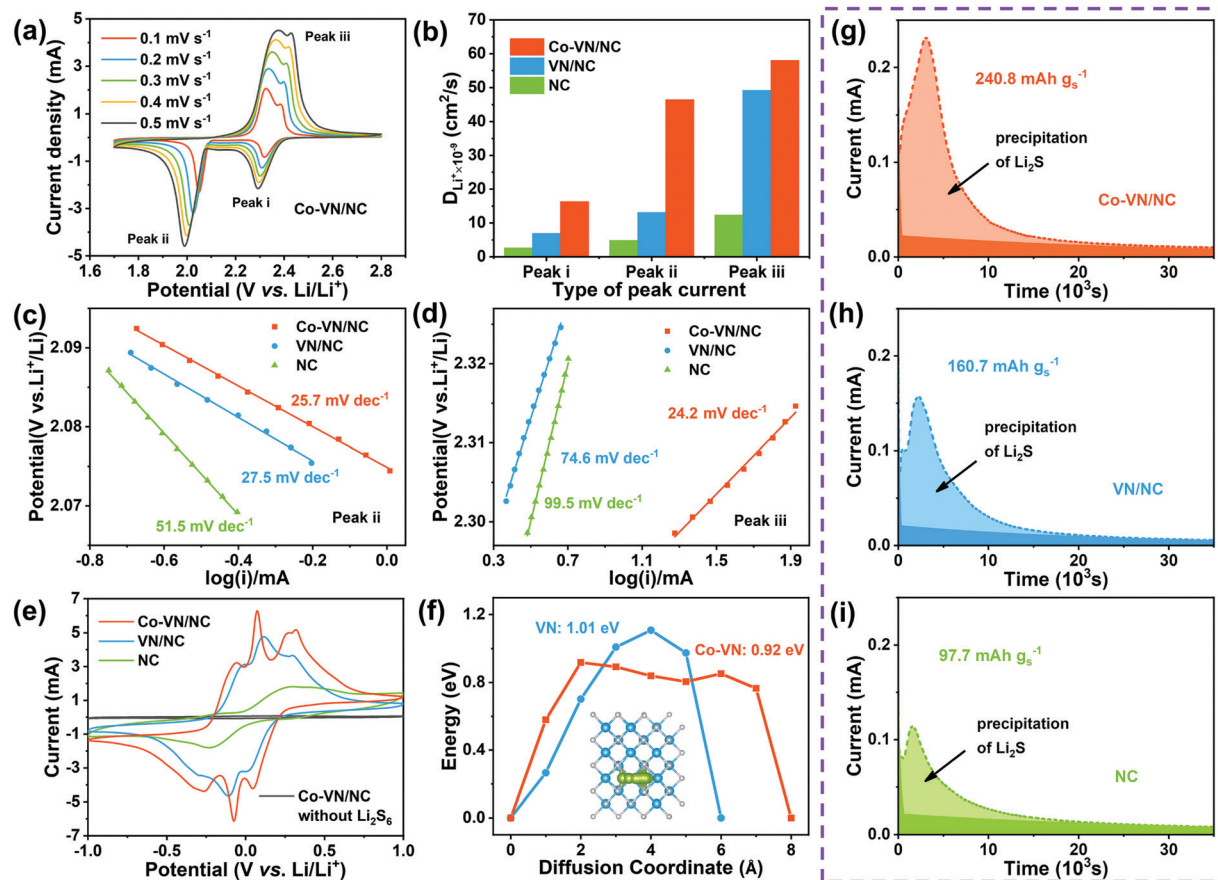
Fig. 5 (a) CV curves of Co-VN/NC electrodes at scan rates from 0.1 to 0.5 \text{ mV s}^{-1} . (b) Diffusion coefficient of Li ions of Co-VN/NC, VN/NC and NC electrodes for peak i, ii, and iii processes. (c and d) Tafel plots corresponding to peak ii and iii with the different cathode composites. (e) CV curves obtained at 1 \text{ mV s}^{-1} for the \text{Li}_2\text{S}_6 symmetric cells using Co-VN/NC, VN/NC and NC as electrodes, respectively. (f) Energy barriers of \text{Li}^+ diffusion on the Co-VN and VN (200) plane. (g–i) Potentiostatic discharge curves of \text{Li}_2\text{S}_8 solution on the surfaces of the Co-VN/NC, VN/NC and NC.
