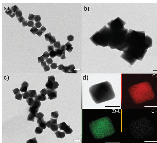
Fig. 7 Representative TEM images of (a) UiO-66 ( \text{ZrOCl}_2 ) (b) UiO-66 ( \text{Cl}^- ) and (c) UiO-66: \text{Cl}^- and (d) EDX elemental mapping of carbon, zirconium and chloride from a UiO-66: \text{Cl}^- NMOF. Scale bars correspond to 200 nm for TEM and to 100 nm for STEM-EDX.
