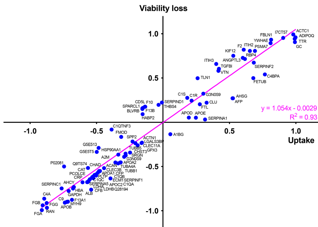
Fig. 10 Role of corona proteins in CD cytotoxicity. Correlation between CD uptake and macrophage viability loss induced by 125\ \mu\text{g mL}^{-1} CDs depending on each top 50 protein present in the NP corona. This analysis was conducted using FACS uptake data for cells exposed to CD1–CD4.
