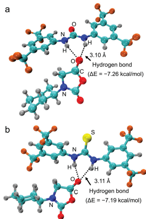
Fig. 5 The DFT-optimized geometry structure showing the hydrogen bonding interaction between (a) U-O and cyclohexyl-NNCA in THF (initier: H, cyan: C, blue: N, red: O, and brown: F), (b) TU-S and cyclohexyl-NNCA in THF (silver: H, cyan: C, blue: N, red: O, yellow: S and brown: F).
