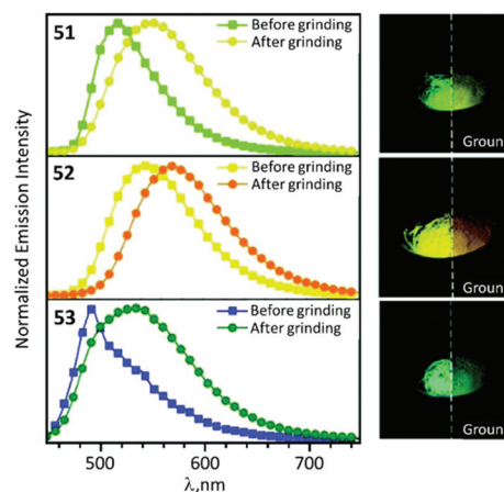
Fig. 11 Solid-state emission spectra of 51–53 before and after grinding using \lambda_{\text{exc}} = 425 nm; photographs taken under UV lamp illumination ( \lambda_{\text{exc}} = 365 nm). Adapted with permission from ref. 49. Copyright (2020) The Royal Society of Chemistry.
