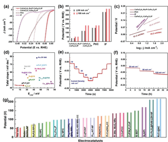
Fig. 3 Electrochemical measurements: (a) HER polarization curves. (b) Overpotential comparison at 50 mA cm -2 and 100 mA cm -2 . (c) Tafel slopes. (d) Comparison of the overpotentials and Tafel slopes with the references. (e and f) Stability tests of the obtained catalysts in 1 M KOH. (g) Comparison of the overpotentials ( E_{100} ) with the reported electrocatalysts.
