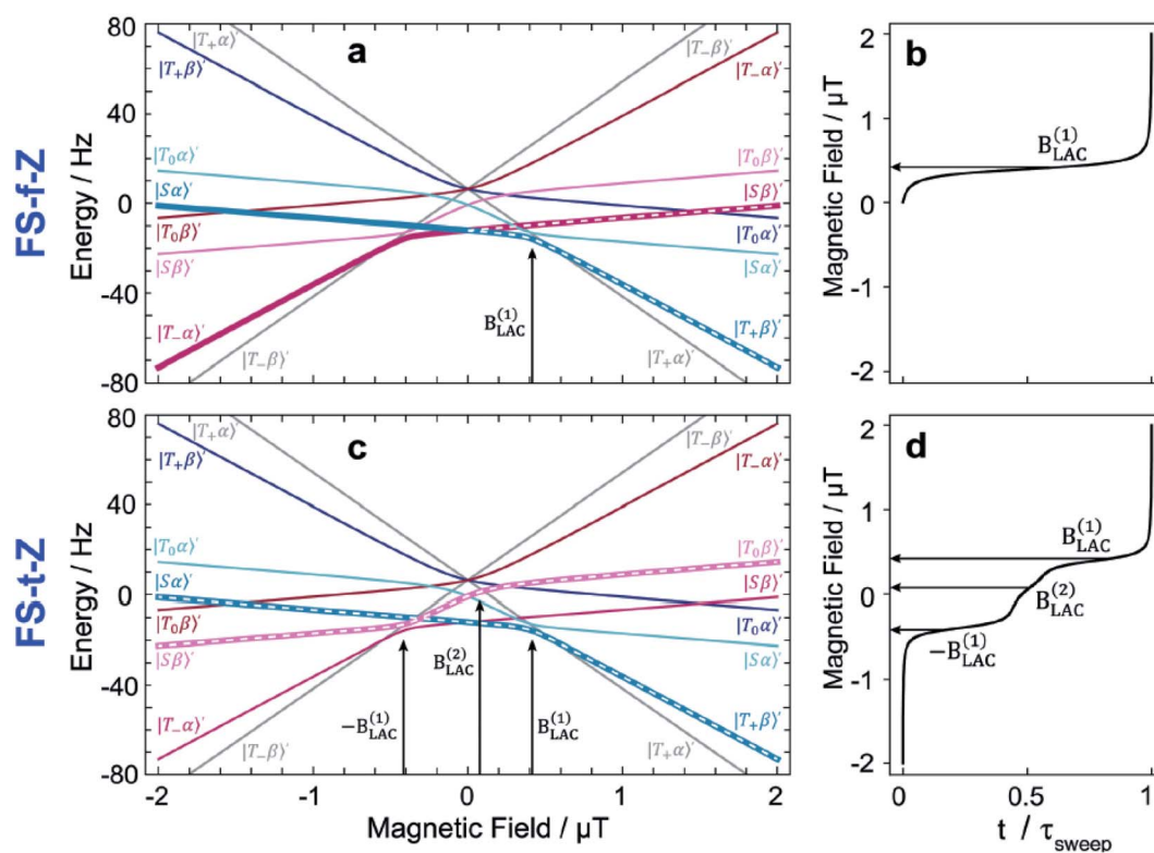
Fig. 7 Eigenvalue plots for the 3-spin system of [1- 13 C]fumarate with state labels shown. (a) Relevant energy levels for the field sweep from zero field (FS-f-Z) experiment are highlighted with white dashes, and the one relevant LAC is labelled. (b) Constant-adiabaticity profile. (c) Relevant energy levels for the field sweep through zero field (FS-t-Z) experiment are highlighted, and the three relevant LACs are labelled. (d) Constant-adiabaticity profile. Colors distinguish between state manifolds with different angular momentum projection (grey: m = \pm 3/2 ; blue: m = +1/2 ; red: m = -1/2 ). For details see Rodin et al. 126 (reproduced from ref. 126 with permission from the Royal Society of Chemistry, copyright 2021).
