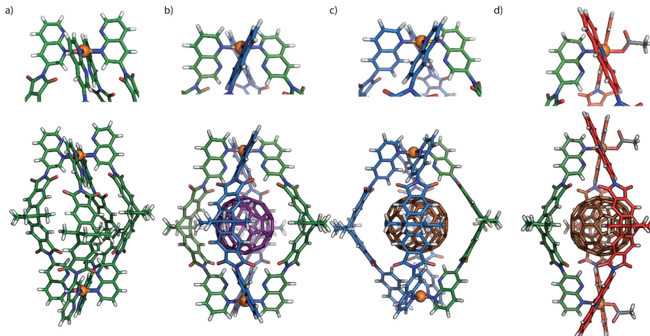
Fig. 5 (a) X-ray structure of [\text{Pd}_2\text{L}^5_4] ; (b) gas-phase B3LYP/LANL2DZ DFT-optimized models of trans - [\text{C}_{60}@\text{Pd}_2\text{L}^2\text{L}^5_2] and (c) [\text{C}_{70}@\text{Pd}_2\text{L}^3\text{L}^5] ; (d) X-ray structure of [\text{C}_{70}@\text{Pd}_2\text{L}^4\text{L}^5(\text{OAc})_2] . Colours: \text{L}^2 : blue, \text{L}^4 : red, \text{L}^5 : green, \text{C}_{60} : purple, \text{C}_{70} : brown. Anions and solvents molecules omitted. For X-ray diffraction and DFT calculation details see ESI.†
