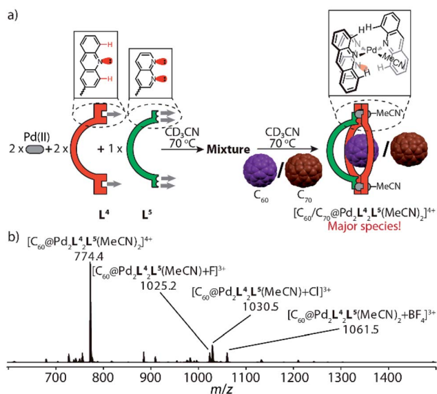
Fig. 6 Self-assembly of fullerene-containing heteroleptic bowl [\text{C}_{60}/\text{C}_{70}@\text{Pd}_2\text{L}^4\text{L}^5(\text{MeCN})_2] : (a) ligands \text{L}^4 and \text{L}^5 react with \text{Pd}^{\text{II}} cations in a 2 : 1 : 2 ratio at 70 °C to give a convoluted mixture, followed by the addition of \text{C}_{60} or \text{C}_{70} to produce heteroleptic bowl [\text{C}_{60}/\text{C}_{70}@\text{Pd}_2\text{L}^4\text{L}^5(\text{MeCN})_2] as major species; (b) high-resolution ESI mass spectrum of [\text{C}_{60}@\text{Pd}_2\text{L}^4\text{L}^5(\text{MeCN})_2] and its anion adducts.
