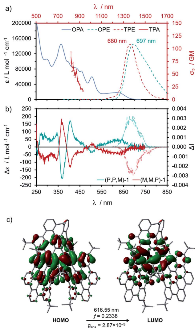
Fig. 3 (a) Experimental OPA (gray), OPE (turquoise, dashed), TPA (red) and TPE (red, dashed) spectra of (M,M,P/P,P,M) -1. Measured in CHCl 3 at ca. 1 × 10 -6 M, λ exc = 370 nm for OPE, λ exc = 900 nm for TPE; (b) experimental ECD spectra of (M,M,P) -1 (red) and (P,P,M) -1 (turquoise) measured in CHCl 3 at ca. 1 × 10 -6 M, and experimental CPL spectra (λ exc = 370 nm) of (M,M,P) -1 (pale red, dashed) and (P,P,M) -1 (pale turquoise, dashed) measured in CHCl 3 at ca. 1 × 10 -6 M; (c) HOMO and LUMO orbitals, and information of the TD-DFT calculated (CAM-B3LYP/6-31G(d,p)) lowest energy transition. The OPE spectrum is cropped at long wavelengths due to the use of a short path filter to block the multiphoton laser at the entrance of the photodetector.
