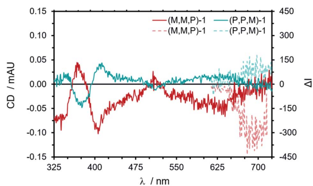
Fig. 4 Experimental ECD spectra of films of (M,M,P) -1 (red) and (P,P,M) -1 (turquoise) and experimental CPL spectra (λ exc = 370 nm) of (M,M,P) -1 (pale red, dotted) and (P,P,M) -1 (pale turquoise, dotted) on quartz substrates from CHCl 3 solutions at ca. 5 mg mL -1 .
