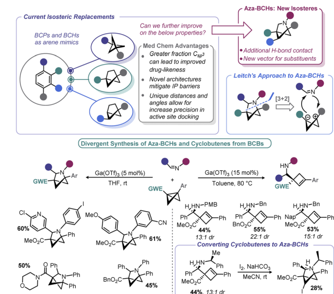
Scheme 13 Leitch's approach to aza-BCHs from BCBs.
