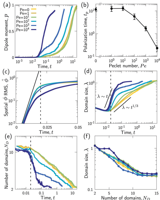
Fig. 3 Advection speeds up droplet polarization by accelerating the coarsening phase. (a) Dipole moment p depending on time for different \text{Pe} . (b) Polarization time t_p as a function of the Peclet number; error bars indicate the standard error of the mean. (c) Spatial root-mean-square of \phi depending on time. The black line shows the initial growth with rate \omega predicted by linear stability analysis, \hat{\phi} \sim e^{\omega t} . (d) Domain size \lambda as defined in the ESI,† depending on time. (e) Number of phase domains N_D depending on time. (f) Domain size \lambda as a function of the number of phase domains N_D . Legends in panels c–f same as in panel a. In panels c–e, the vertical dashed line indicates the approximate end time t_d \approx 0.02\tau_D of the initial decomposition phase. The quantities on all ordinate axes are averaged over 25 simulation runs.
