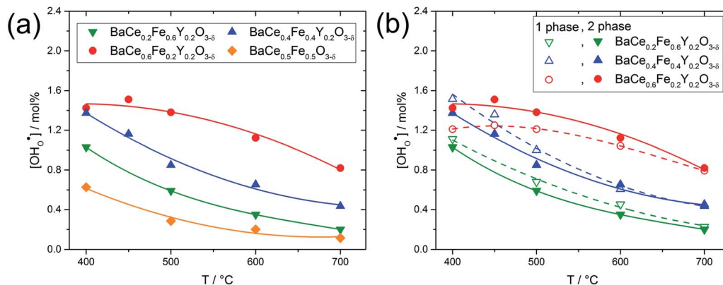
Fig. 5 (a) Proton concentrations of two-phase composites with frozen-in oxygen stoichiometry in 17 mbar p\text{H}_2\text{O} (samples were quenched from 700 °C in \text{N}_2 ) as a function of temperature. (b) Comparison of the proton concentration of two-phase composites (samples sintered at temperatures below the upper critical mixing temperature; closed symbols and full lines) and the corresponding single phases (samples sintered at temperatures above the upper critical mixing temperature; open symbols and dashed line). The lines are guidelines to the eye.
