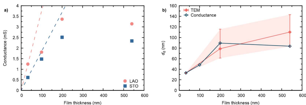
Fig. 6 (a) Measured equilibrium conductance by Van-der-Pauw measurements at 375 °C in high p_{\text{O}_2} . Dashed lines are extrapolations of the expected conductance of a fully dense layer. (b) Thickness of the dense bottom layer, d_d , for L2NO4/LAO samples, estimated from conductance measurements assuming constant conductivity and via TEM measurements. Filled area indicates observed variations of the dense layer thickness by TEM, e.g. minimum and maximum values.
