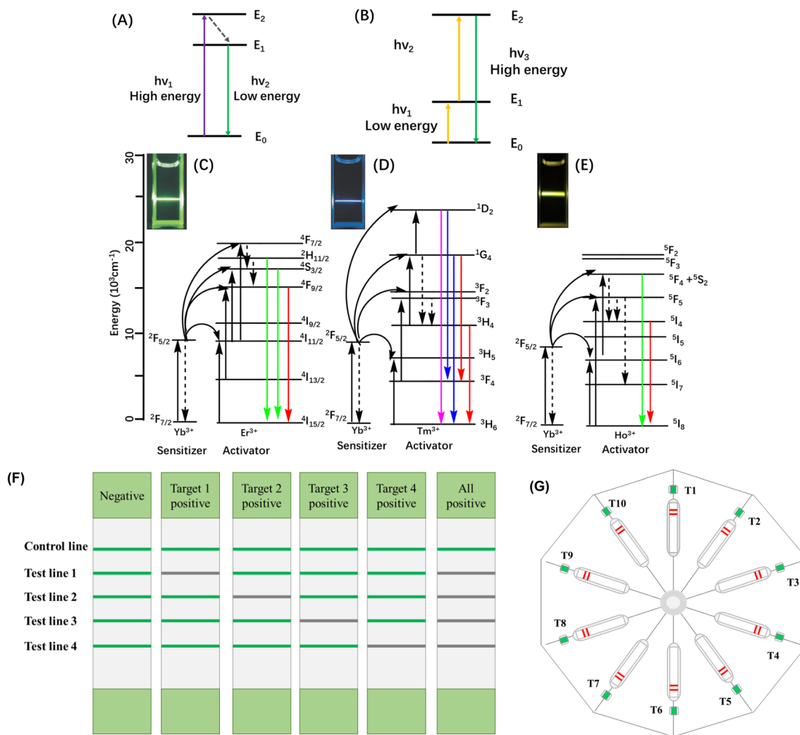
Fig. 10 Schematic principle of (A) conventional photoluminescence and (B) the mechanism of the upconversion luminescence process of the lanthanide UCNPs co-doped with (C) Yb^{3+} and Er^{3+} , (D) Yb^{3+} and Tm^{3+} , and (E) Yb^{3+} and Ho^{3+} . Figure adapted from Zhou et al. , Chem. Rev. , 2015, 115, 10575–10636. (F) Lateral flow strips for the simultaneous detection of four different types of targets. Figure adapted from Chen et al. , Biosens. Bioelectron. , 2016, 79, 430–434. (G) A sketch map of a multi-channel test disk. Figure adapted from Hong et al. , J. Microbiol. Methods , 2010, 83, 133–140. There are 10 strip-holding channels arranged on the base in the central symmetry.
