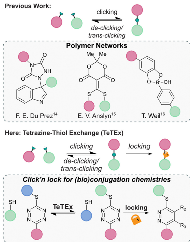
Fig. 1 Previous reports of reversible conjugation chemistries found in the context of polymer networks. From left to right; ene adduct of 1,2,4-triazolone-3,5-diones with indoles, thiols added to a Meldrum's acid-based conjugate acceptor, and click chemistry adduct between boronic acids and diols. 14–16 Here, we report tetrazine–thiol exchange TeTEX as a fully reversible click reaction between non-symmetric thiol functionalized tetrazines and thiol substrates for the modification of functionalized biomolecules. On-demand locking with a bioorthogonal stimulus provides a switch from reversibility to irreversibility.
