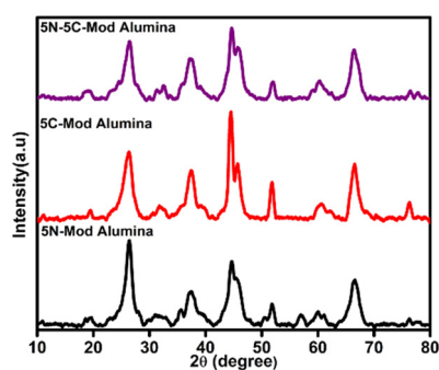
Fig. 9 XRD profile of spent 5Ni-mod alumina, 5Co-mod alumina, and 5Ni-5Co-mod alumina catalysts.
