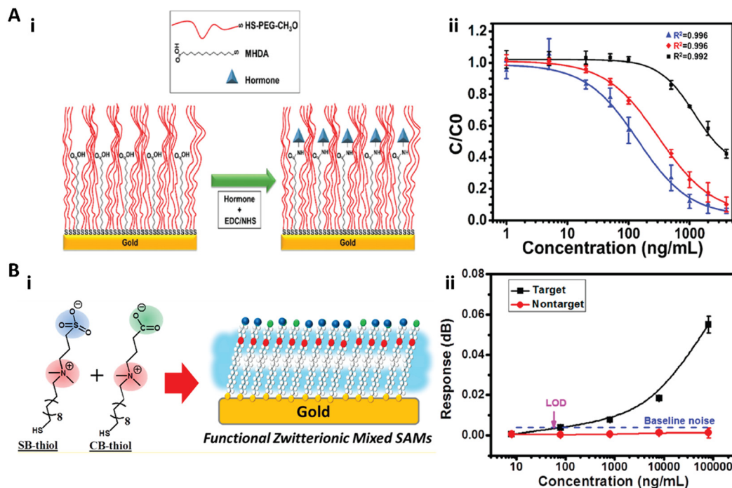
Fig. 2 A-i) The schematic illustration of the mixed SAM formed on the Au film. The thiolated polyethylene glycol ( \text{CH}_2\text{O}-\text{PEG}-\text{SH} ) in the mixed SAM served as the spacer and the antifouling agent to prevent the nonspecific adsorption, while the 16-mercaptohexadecanoic acid (MHDA) was used for hormone immobilization. A-ii) Multiplex hormone calibration curves of the SPR sensor for insulin (blue), glucagon (red), and somatostatin (black). Reproduced from ref. 56, Copyright 2018 American Chemical Society. B-i) The schematic illustration of the functional zwitterionic mixed SAMs with sulfobetaine-thiol (SB-thiol) and carboxybetaine-thiol (CB-thiol). B-ii) Calibration curve for detection of the target and nontarget secondary antibodies with the SPR biosensor. Reproduced from ref. 61, Copyright 2019 American Chemical Society.
