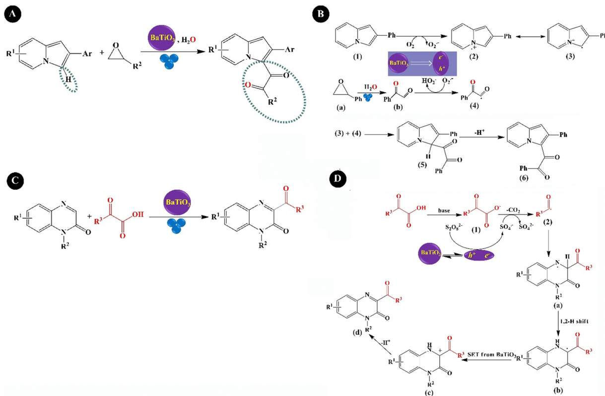
Fig. 11 The mechano-induced synthesis procedure (A) and mechanism (B) of 1,2-diketoindolizine from indolizines and epoxides over \text{BaTiO}_3 (adapted from ref. 211 with permission from American Chemical Society). The mechano-induced synthesis (C) and mechanism (D) of C3-acylation quinoxalin-2(1H)-ones (adapted from ref. 213 with permission from American Chemical Society).
